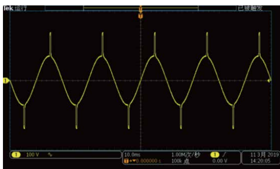
Surge
