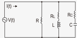
Parallel rlc
