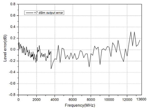
Measured at +7 dBm, level error vs frequency
