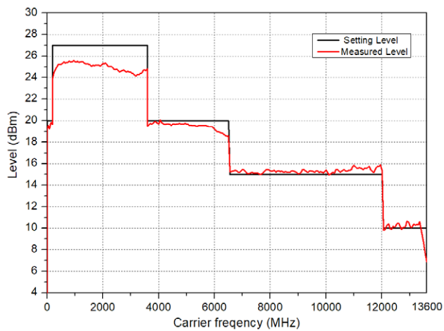
Measured maximum level, Level vs frequency
