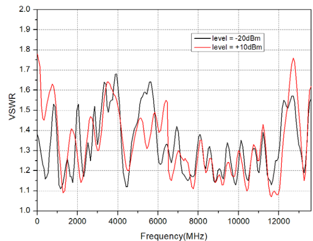
Measured VSWR, VSWR vs frequency
