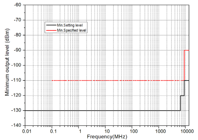
Minimum output level vs frequency
