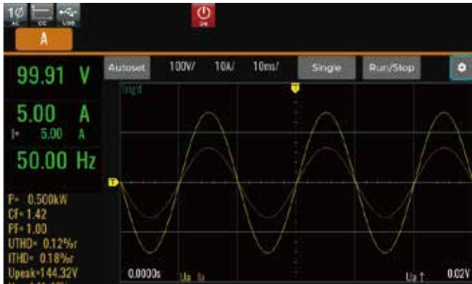
CC mode,CF=1.414
